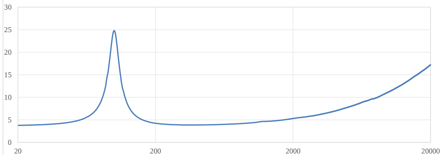
4inch speaker without box-1W/1m
